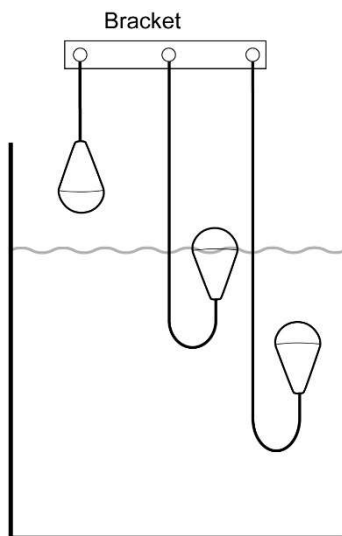
Fig. 5 Correct hydraulic installation
